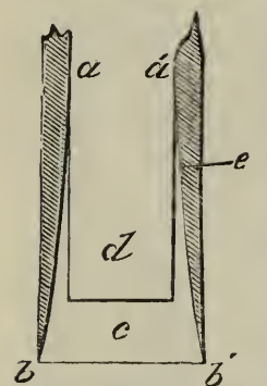
Fig. 194.—Base of peg-box prepared to splice on to neck.
